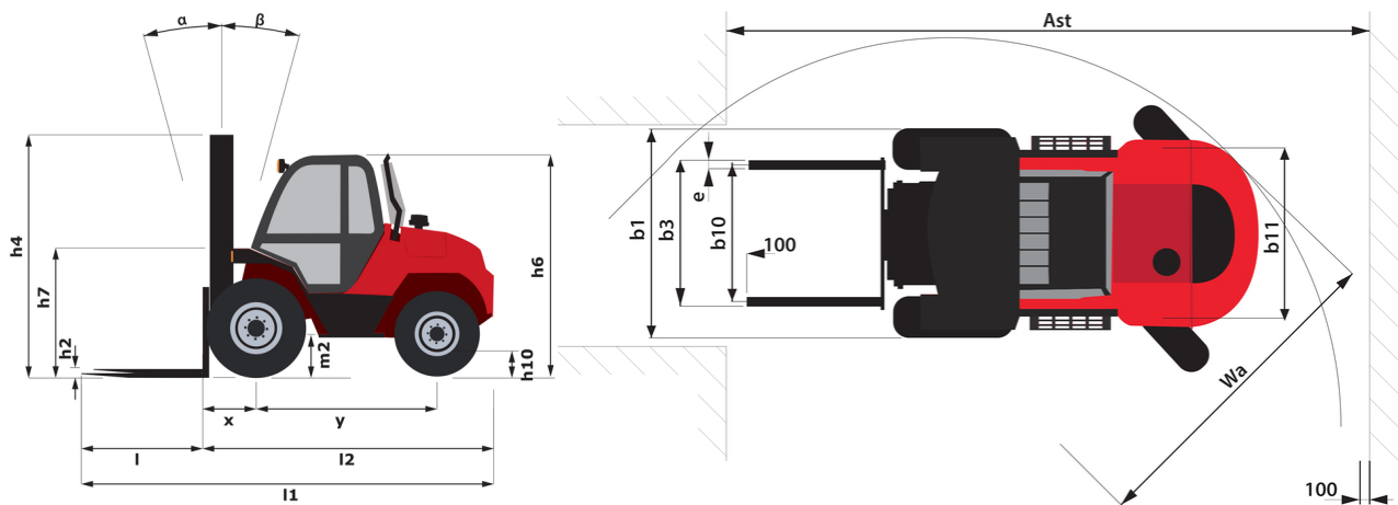
M-X 70-2 - Diagrama dimensional
